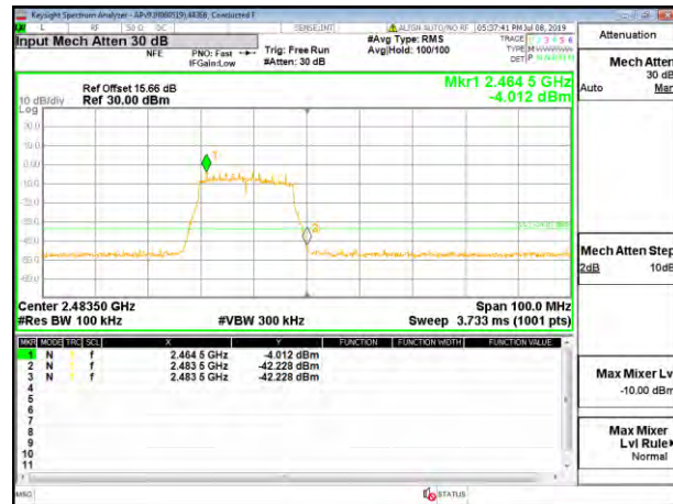
HIGH CHANNEL 13 BANDEGE ANT 2
