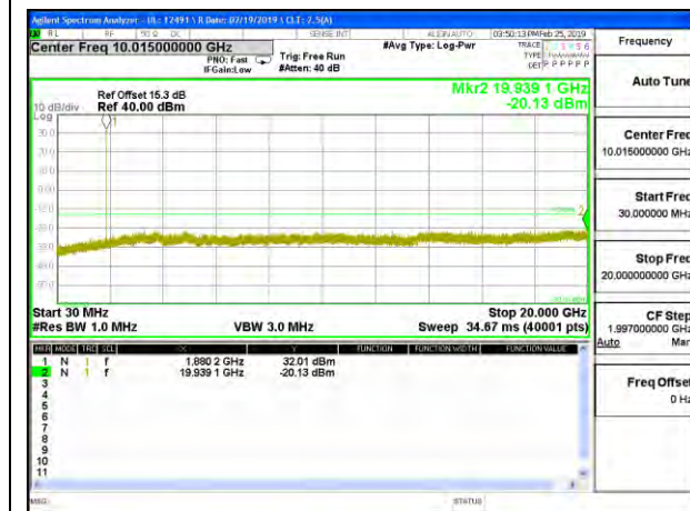
GSM 1900MHz GPRS Middle Channel
