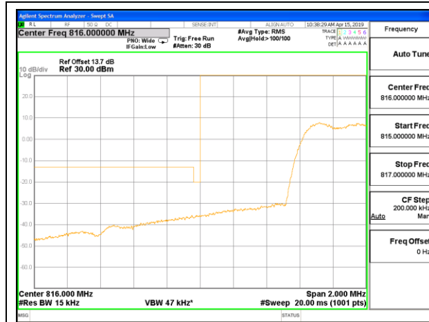
CDMA BC10 1xRTT Low Channel, RBW=1% of EBW ID:39919
