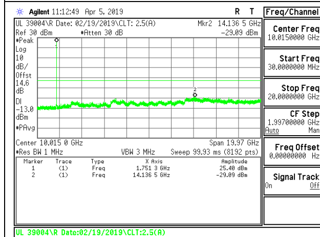
WCDMA Band 4 Rel 99 High Channel
