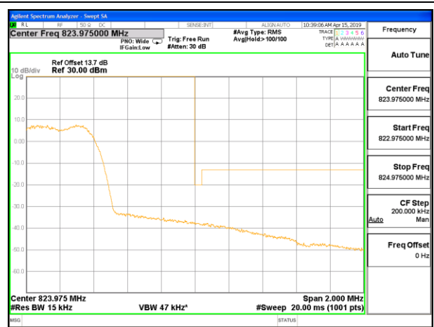
CDMA BC10 1xRTT High Channel, RBW=1% of EBW ID:39919
