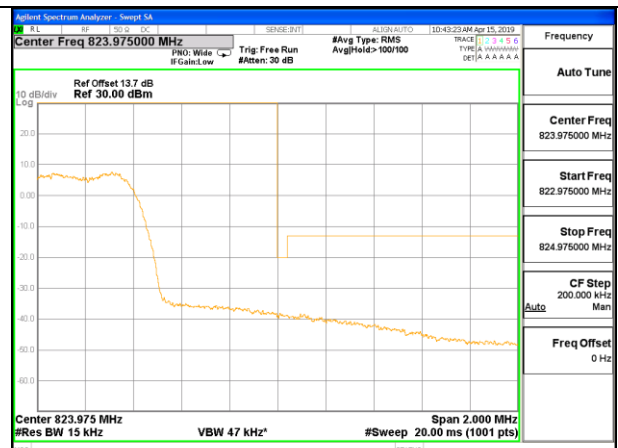
CDMA BC10 1xEV-DO Rev A High Channel, RBW=1% of EBW ID:39919
