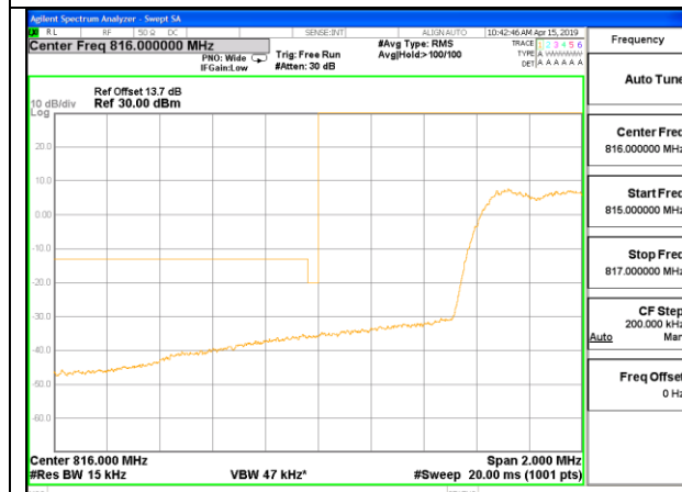
CDMA BC10 1xEV-DO Rev A Low Channel, RBW=1% of EBW ID:39919
