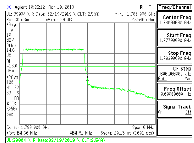
LTE B66 3MHz 16QAM High Channel RB15-0
