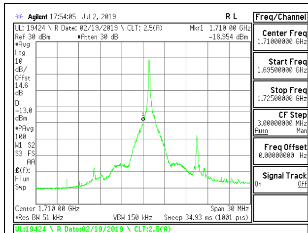
LTE B66 15MHz 16QAM Low Channel RB1-0 not the peak one
