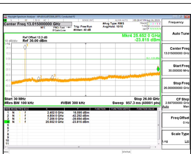
LOW CHANNEL OUT-OF-BAND ANT 4
