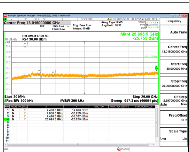
HIGH CHANNEL OUT-OF-BAND ANT 4
