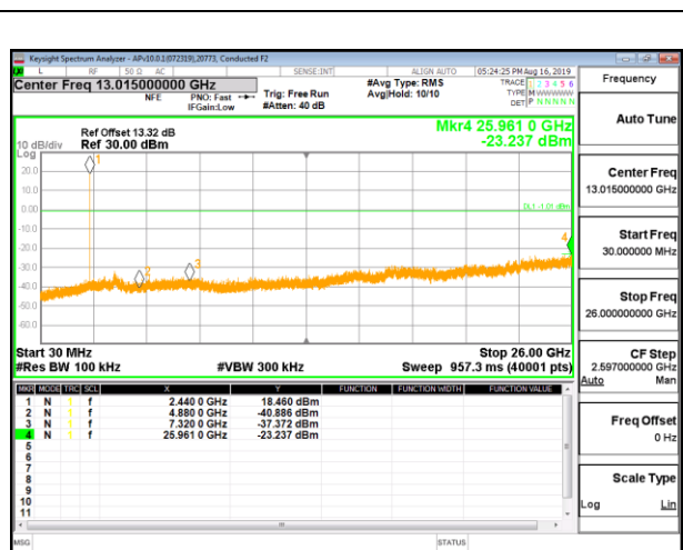
MID CHANNEL OUT-OF-BAND ANT 4
