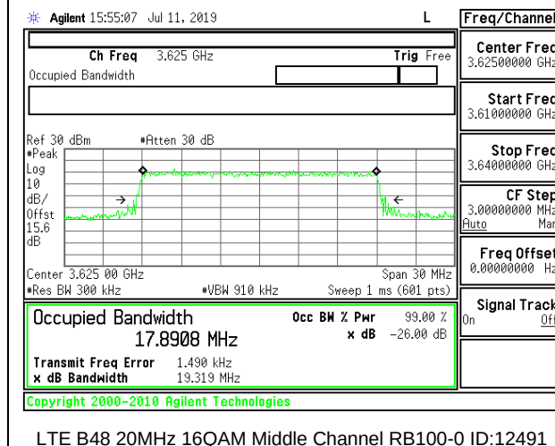
LTE B48 20MHz 16QAM Middle Channel RB100-0 ID:12491
