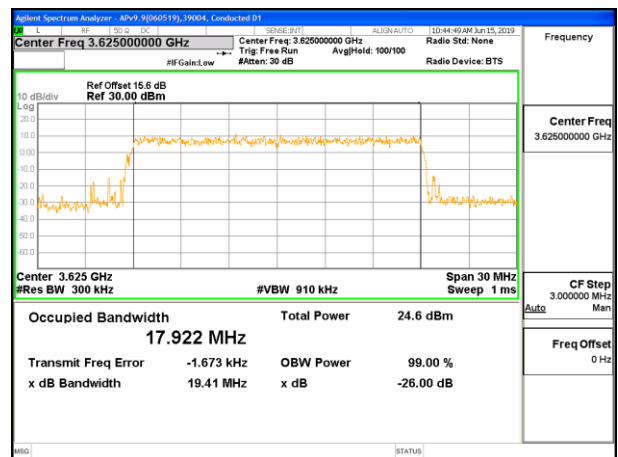
LTE B48 20MHz 64QAM Middle Channel RB100-0
