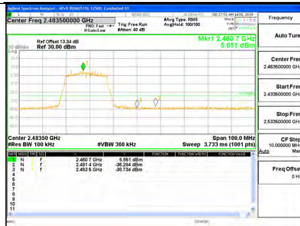
HIGH CHANNEL 11 BANDEDGE ANTENNA 3
