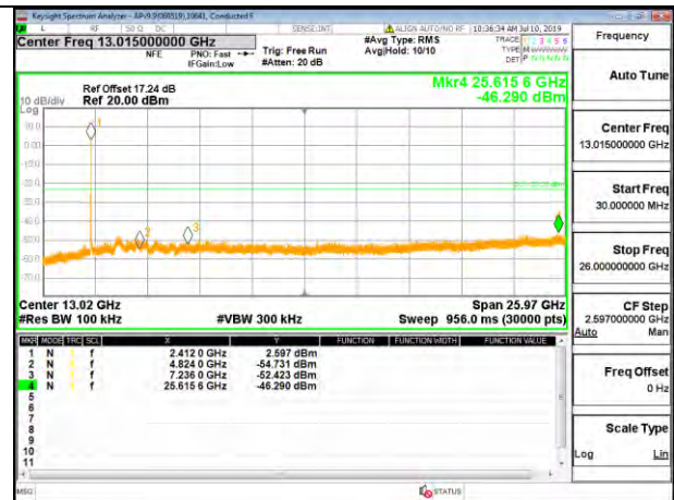
OUT-OF-BAND LOW CHANNEL 1 ANTENNA 4
