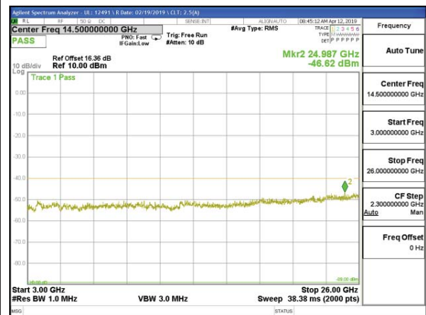
LTE B30 10MHz QPSK Middle Channel RB1-0
