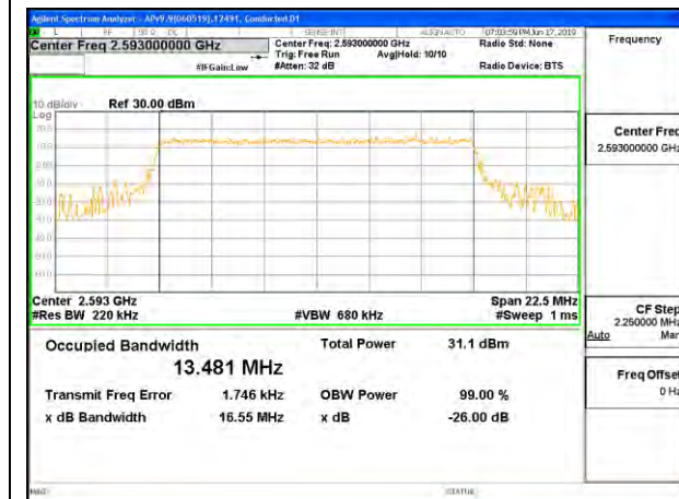
LTE B41 15MHz 64QAM Middle Channel RB75-0
