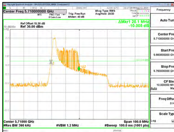
CHANNEL 142 ANTENNA 5
