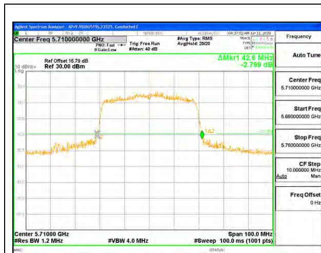
CHANNEL 142 ANTENNA 6
