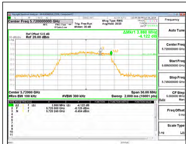
CHANNEL 144 ANTENNA 6
