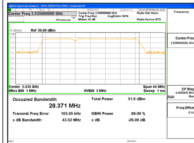
LTE B7 10MHz + 20MHz 64QAM RB50-0 + RB100-0
