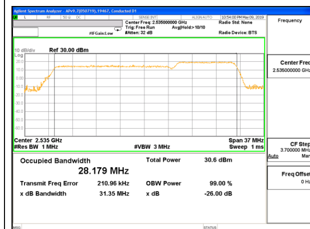
LTE B7 20MHz + 10MHz 16QAM RB100-0 + RB50-0
