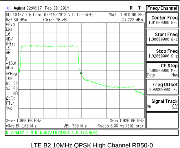
LTE B2 10MHz QPSK High Channel RB50-0
