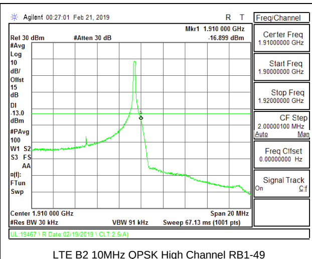
LTE B2 10MHz QPSK High Channel RB1-49
