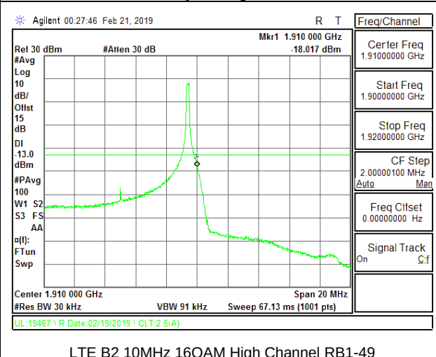
LTE B2 10MHz 16QAM High Channel RB1-49
