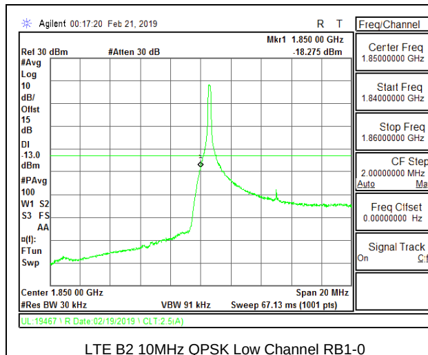
LTE B2 10MHz QPSK Low Channel RB1-0
