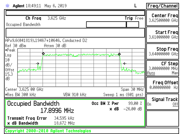
LTE B48 20MHz QPSK Middle Channel RB50-0
