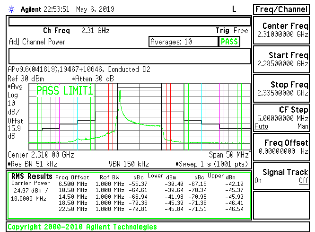
LTE B30 10MHz 16QAM Middle Channel RB1-0
