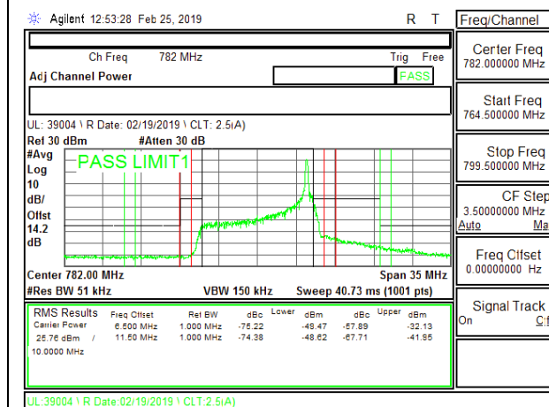
LTE B13 10MHz QPSK Middle Channel RB1-49
