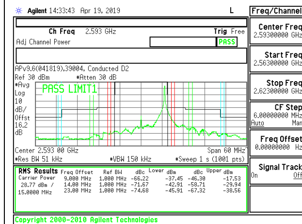
LTE B41 15MHz QPSK Middle Channel RB1-74
