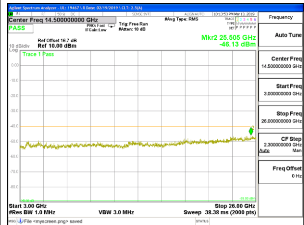
LTE B30 5MHz 16QAM Low Channel RB1-0
