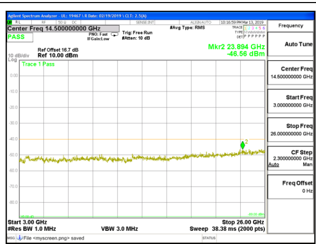
LTE B30 5MHz 16QAM Middle Channel RB1-0
