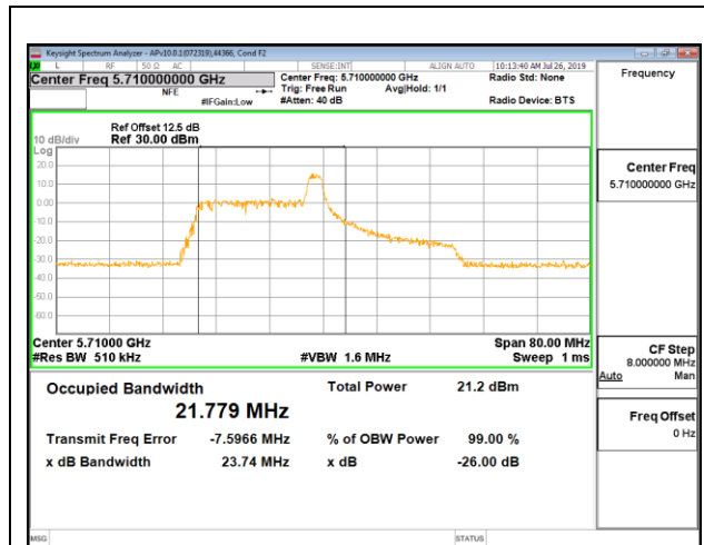
CHANNEL 142 ANT 4
