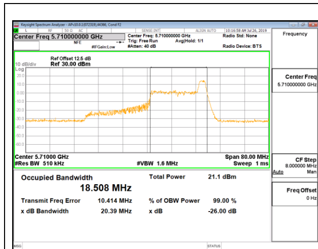
CHANNEL 142 ANT 4
