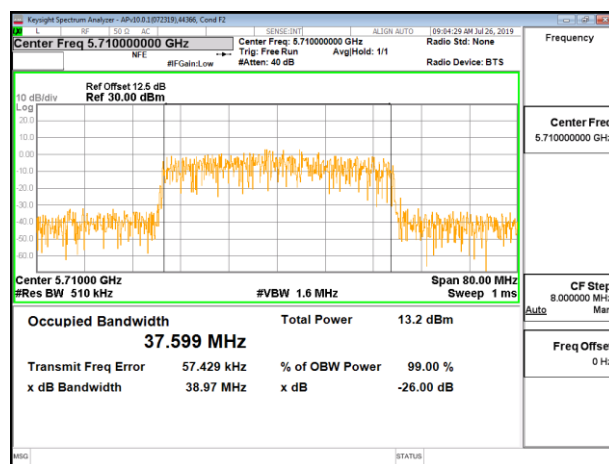
CHANNEL 142
