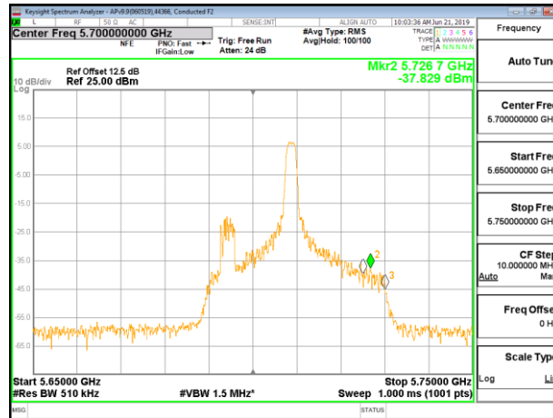
CHANNEL 142 PSD
