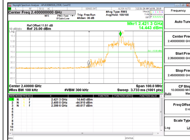
LOW CHANNEL 3 BANDEGE ANT 5
