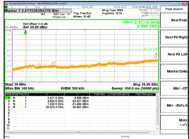
OUT-OF-BAND LOW CHANNEL 1 ANT 5
