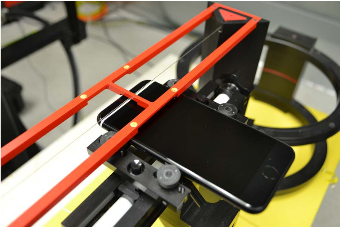
Setup Photo Front View of the DUT
