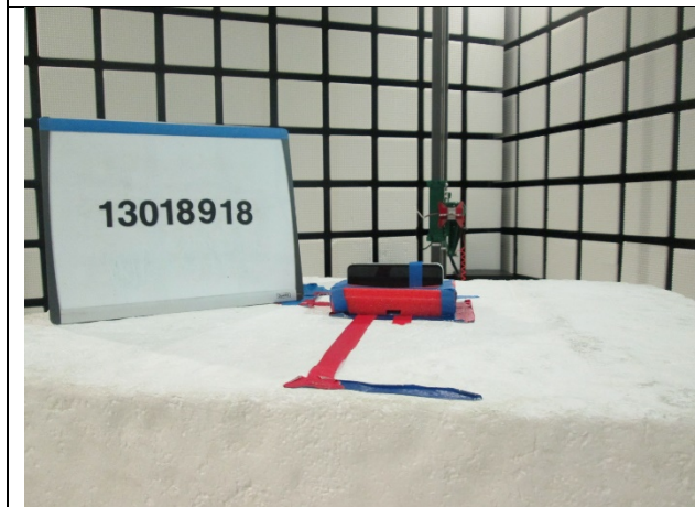
Y-Axis Front
