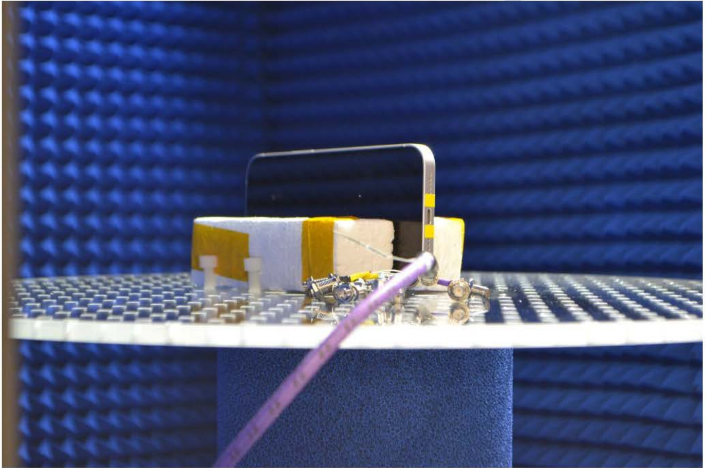
Figure C-5 Radiated power mmW test measurement setup
