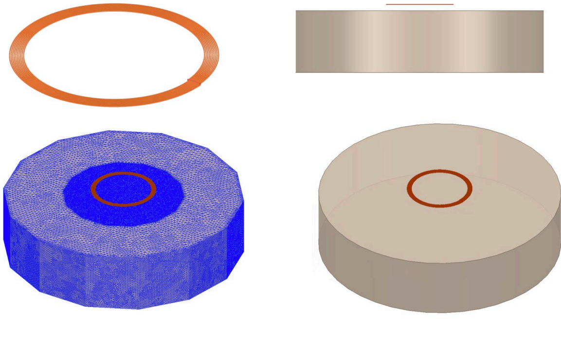
Figure 4: Current loop in front of a cuboid
