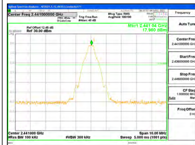
MID CHAANEL BANDEDGE
