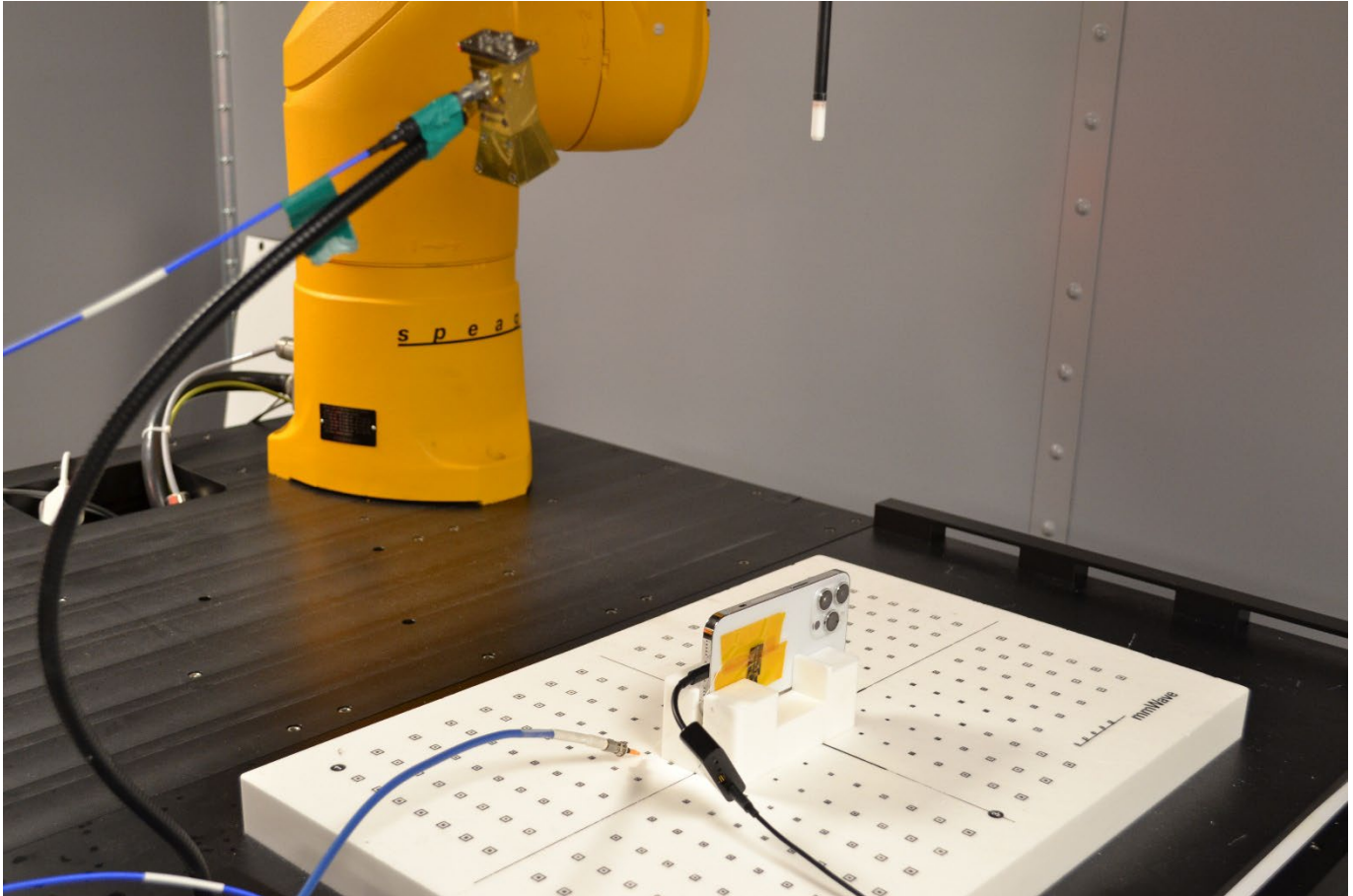
Figure C- 5 DASY radiated power mmW test measurement setup
