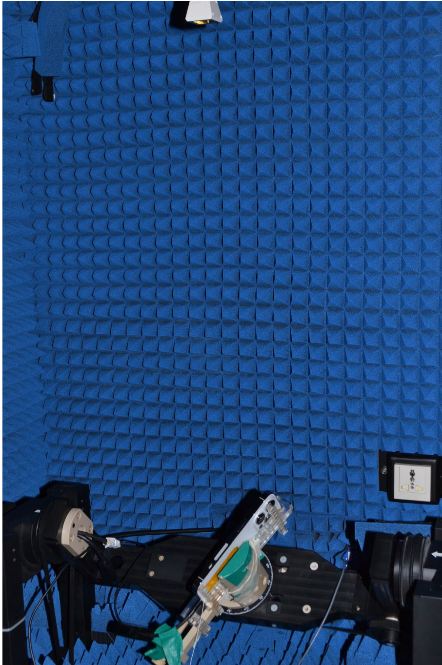
Figure C-6 Radiated power mmW test measurement setup
