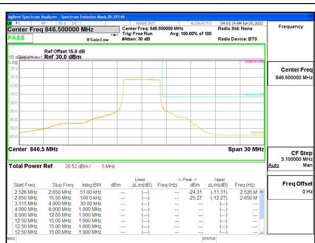
LTE B5 5MHz QPSK High Channel RB25-0
