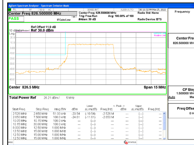
5G NR n5 5MHz BPSK Low Channel RB25-0, ID 28774
