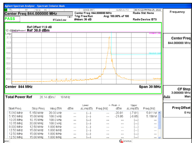
5G NR n5 10MHz BPSK High Channel RB1-51, ID 28774
