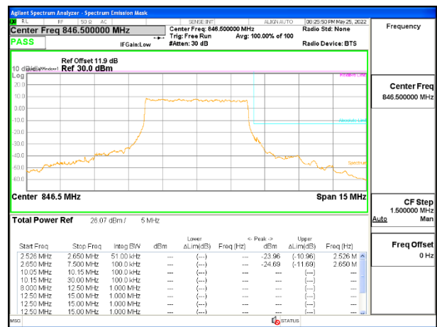
5G NR n5 5MHz BPSK High Channel RB25-0, ID 28774
