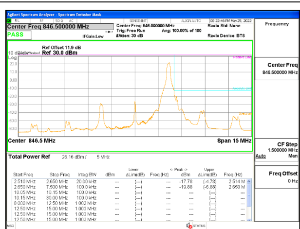
5G NR n5 5MHz BPSK High Channel RB1-24, ID 28774
