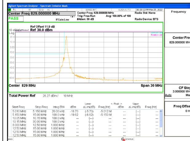
5G NR n5 10MHz BPSK Low Channel RB1-0, ID 28774
