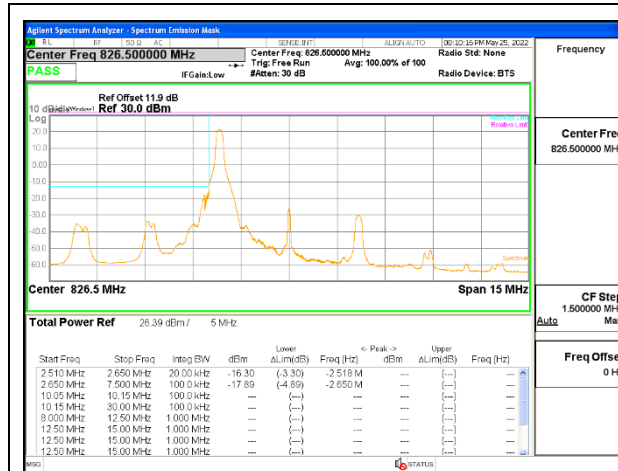
5G NR n5 5MHz BPSK Low Channel RB1-0, ID 28774
