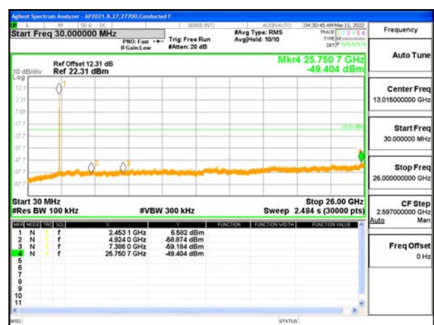
HIGH CHANNEL 11 OUT-OF-BAND [ANT 3]
