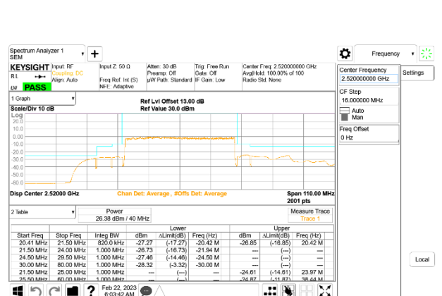
5G NR n7 40MHz BPSK Low Channel RB216-0, ID:27957
