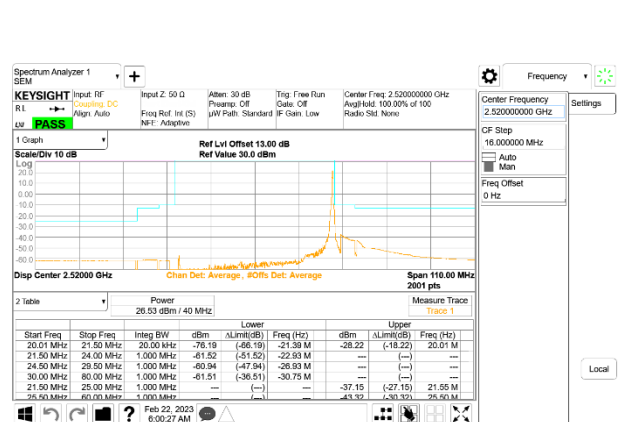
5G NR n7 40MHz BPSK Low Channel RB1-215, ID:27957
