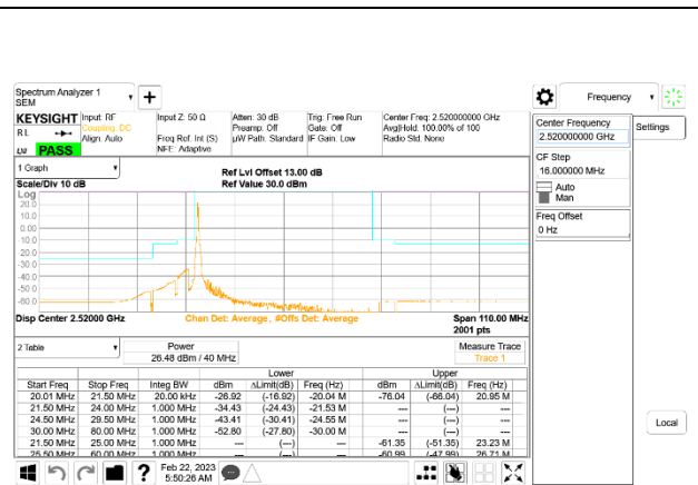
5G NR n7 40MHz BPSK Low Channel RB1-0, ID:27957
