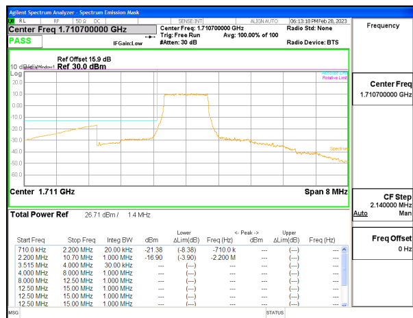
LTE B66 1.4MHz QPSK Low Channel RB6-0, ID:25780
