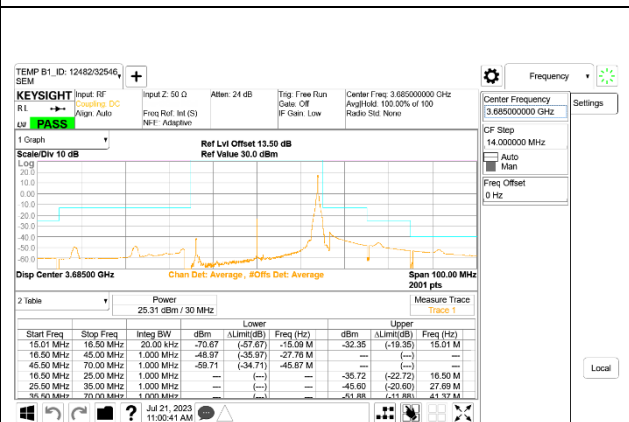
5G NR n48 30MHz BPSK High Channel RB1-77
