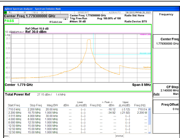
LTE B66 1.4MHz QPSK High Channel RB1-5, ID:25780
