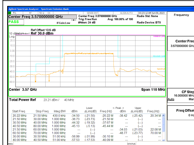
5G NR n48 40MHz BPSK Low Channel RB100-0, ID:12482
