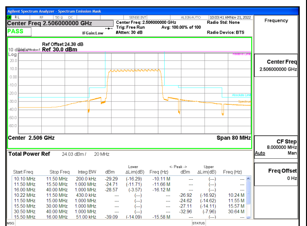
LTE B41 20MHz QPSK Low Channel RB100-0 ID:19210
