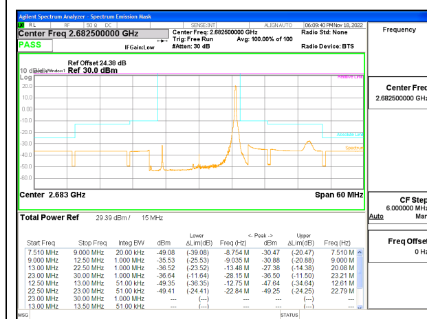
LTE B41 15MHz QPSK High Channel RB1-74 ID:19210
