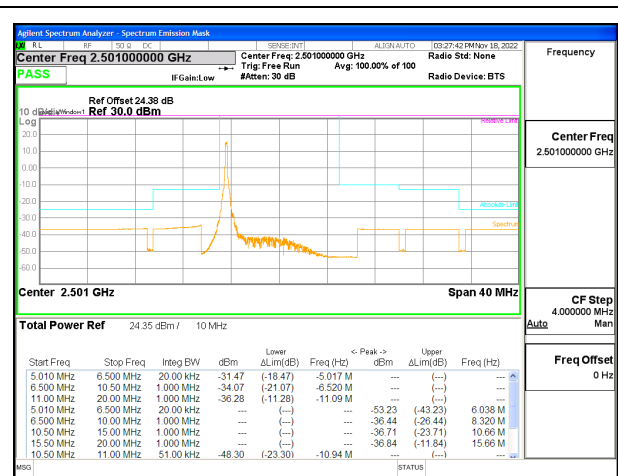
LTE B41 10MHz QPSK Low Channel RB1-0 ID:19210
