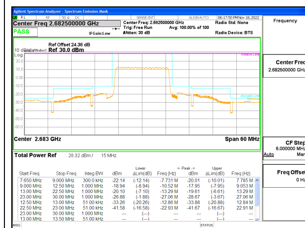
LTE B41 15MHz QPSK High Channel RB75-0 ID:19210
