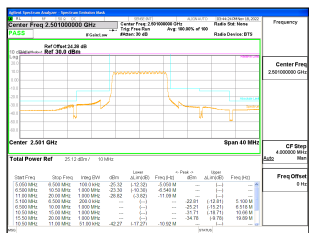
LTE B41 10MHz QPSK Low Channel RB50-0 ID:19210
