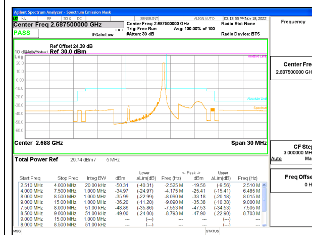
LTE B41 5MHz QPSK High Channel RB1-24 ID:19210
