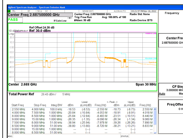
LTE B41 5MHz QPSK High Channel RB25-0 ID:19210
