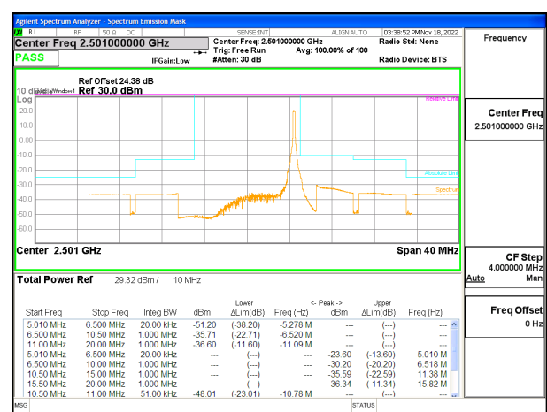
LTE B41 10MHz QPSK Low Channel RB1-49 ID:19210
