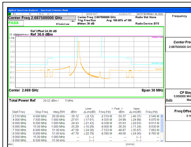
LTE B41 5MHz QPSK High Channel RB1-0 ID:19210
