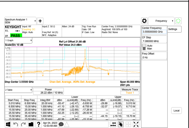
LTE B48 10MHz QPSK Low Channel RB1-49, ID:28567
