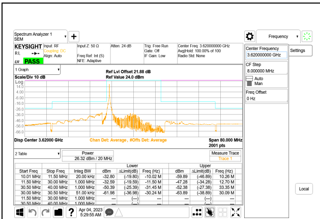
LTE B48 20MHz QPSK Middle Channel RB1-0, ID:28567
