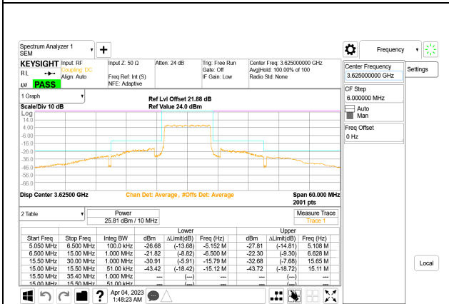
LTE B48 10MHz QPSK Middle Channel RB50-0, ID:28567
