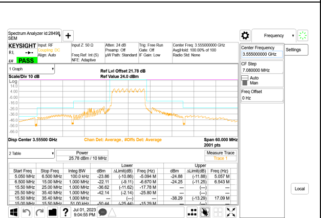
LTE B48 10MHz QPSK Low Channel RB50-0, ID:28567
