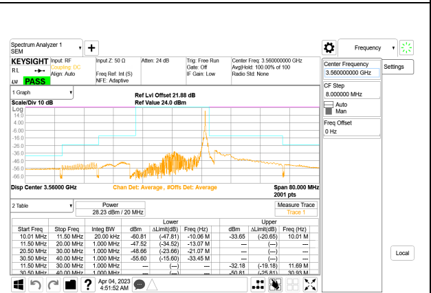
LTE B48 20MHz QPSK Low Channel RB1-99, ID:28567
