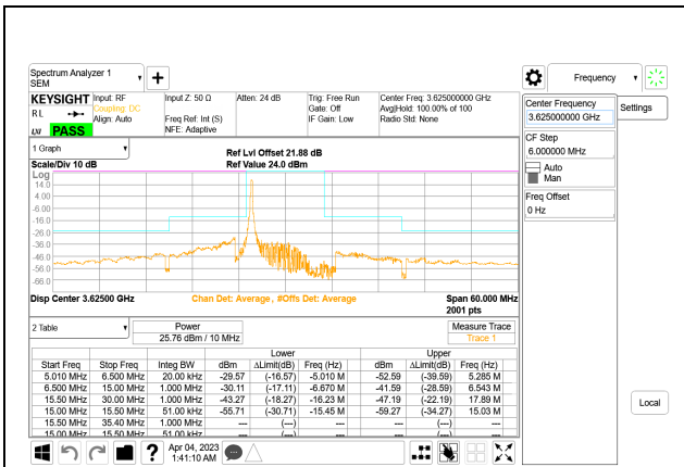
LTE B48 10MHz QPSK Middle Channel RB1-0, ID:28567
