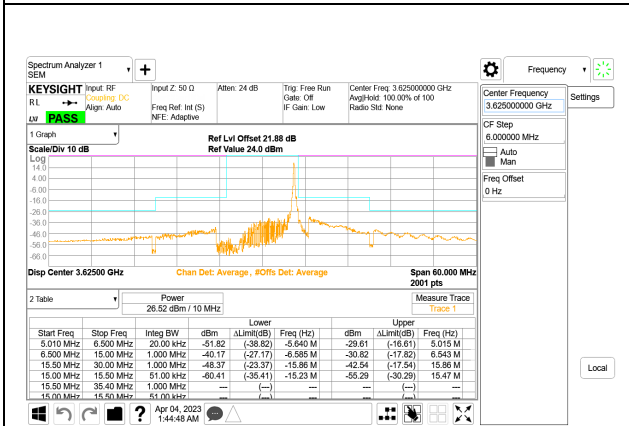
LTE B48 10MHz QPSK Middle Channel RB1-49, ID:28567
