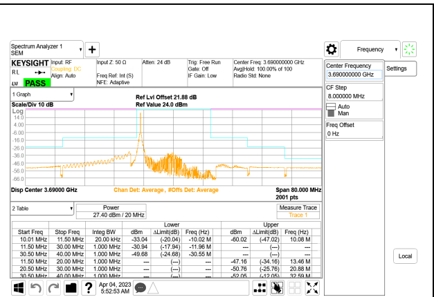
LTE B48 20MHz QPSK High Channel RB1-0, ID:28567
