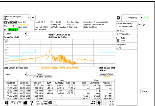
LTE B48 20MHz QPSK Low Channel RB1-0, ID:28567
