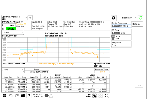
LTE B48 20MHz QPSK Low Channel RB100-0, ID:28498
