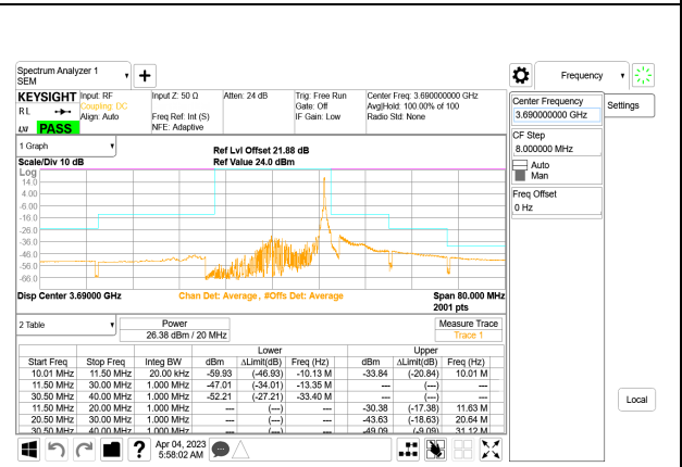
LTE B48 20MHz QPSK High Channel RB1-99, ID:28567
