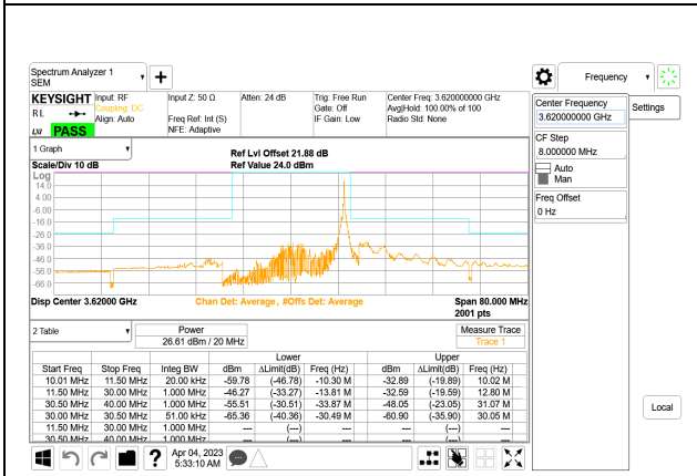
LTE B48 20MHz QPSK Middle Channel RB1-99, ID:28567
