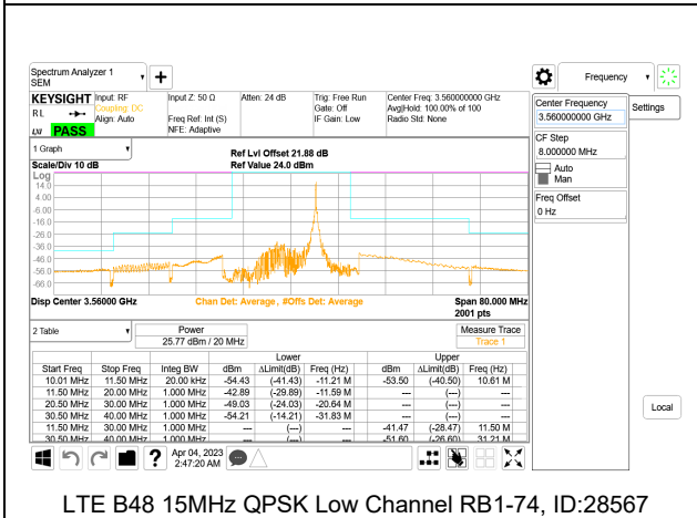
LTE B48 15MHz QPSK Low Channel RB1-74, ID:28567
