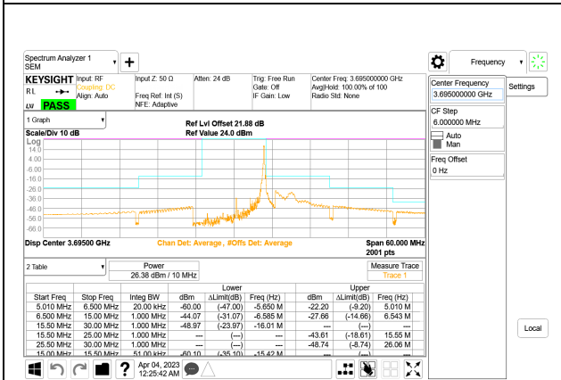
LTE B48 5MHz QPSK High Channel RB1-24, ID:28567
