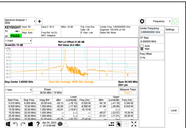
LTE B48 10MHz QPSK High Channel RB1-0, ID:28567
