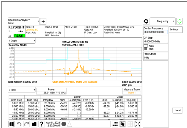
LTE B48 5MHz QPSK High Channel RB1-0, ID:28567
