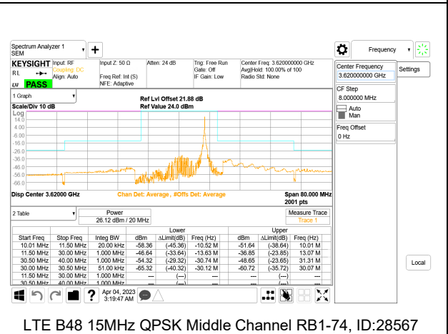
LTE B48 15MHz QPSK Middle Channel RB1-74, ID:28567
