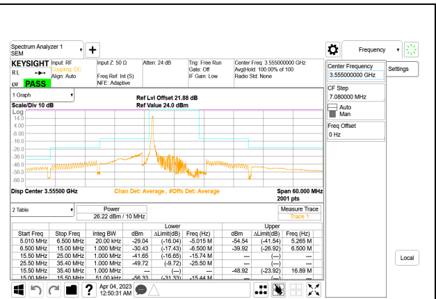
LTE B48 10MHz QPSK Low Channel RB1-0, ID:28567
