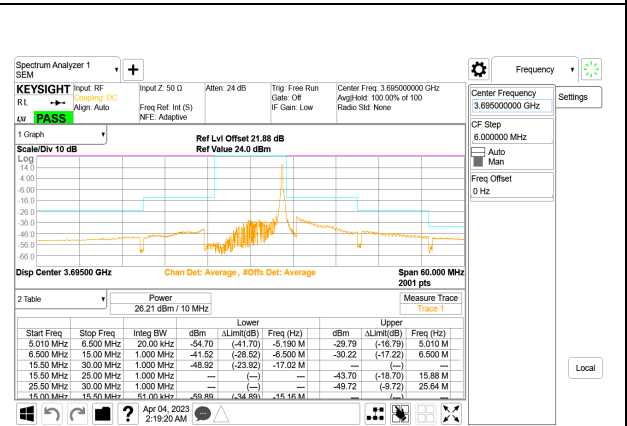
LTE B48 10MHz QPSK High Channel RB1-49, ID:28567
