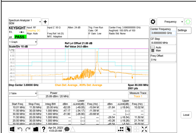
LTE B48 15MHz QPSK High Channel RB1-74, ID:28567
