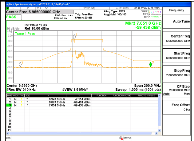
LOW CHANNEL 6965
