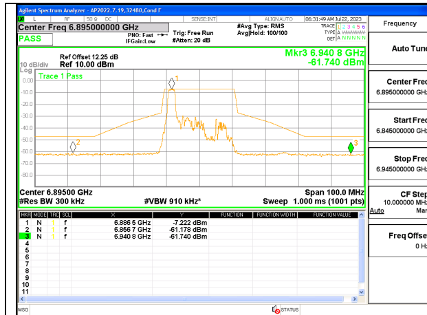
LOW CHANNEL 6895
