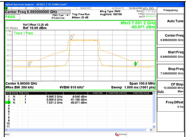
MID CHANNEL 6995
