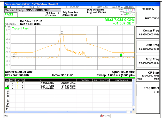
MID CHANNEL 6995
