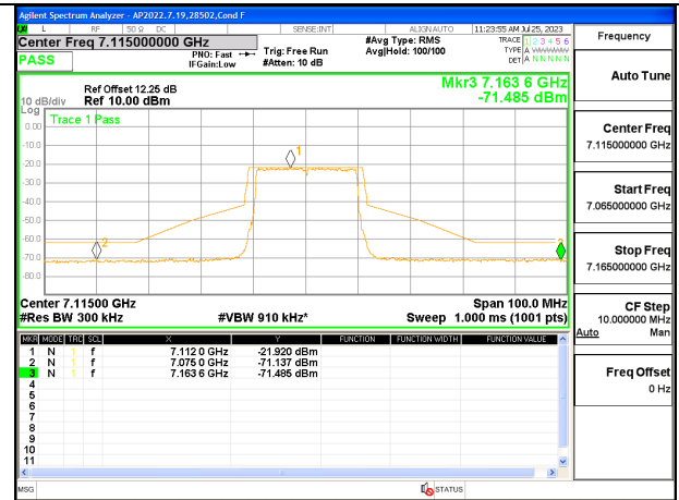
233 CHANNEL 7115
