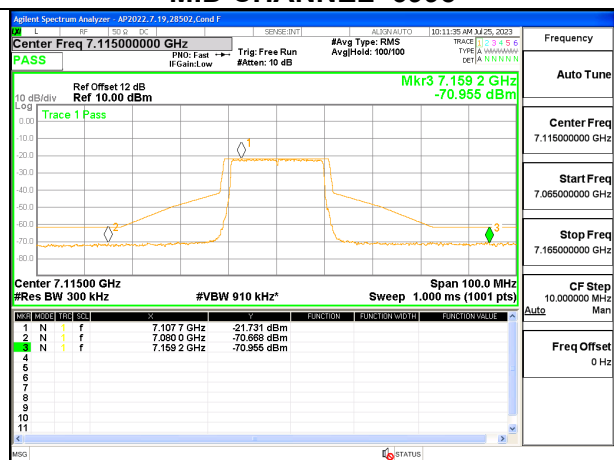
233 CHANNEL 7115
