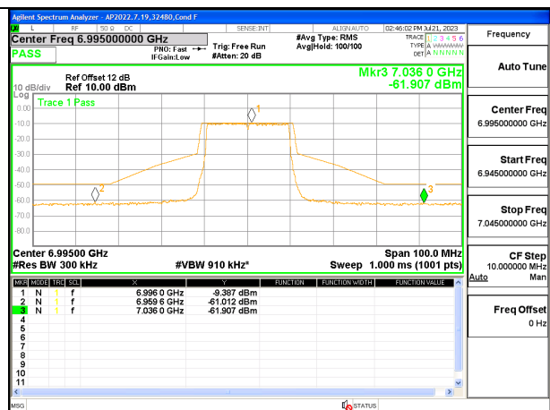
MID CHANNEL 6995
