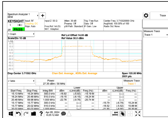
5G NR n77 30MHz BPSK Low Channel RB75-0 Port A ID 27342
