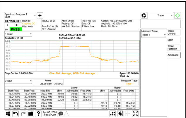
5G NR n77 30MHz BPSK Mid Channel RB75-0 Port A ID 27342
