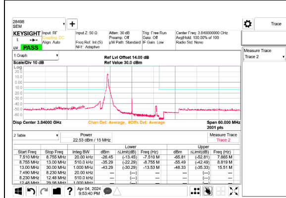
5G NR n77 15MHz BPSK Middle Channel RB1-0 Port B
