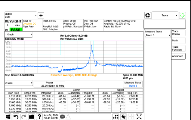
5G NR n77 15MHz BPSK Mid Channel RB1-37 Port A+B
