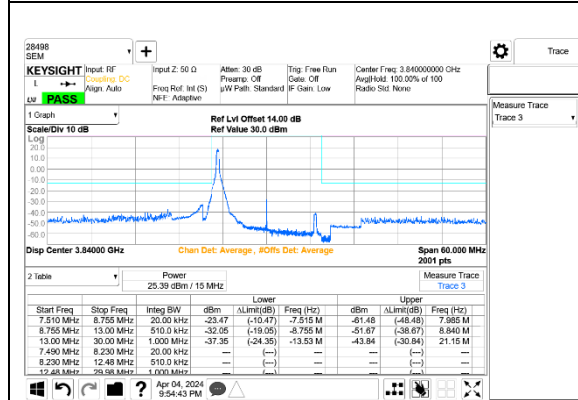
5G NR n77 15MHz BPSK Middle Channel RB1-0 Port A+B
