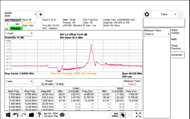
5G NR n77 15MHz BPSK Mid Channel RB1-37 Port B
