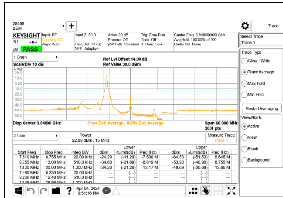
5G NR n77 15MHz BPSK Middle Channel RB1-0 Port A
