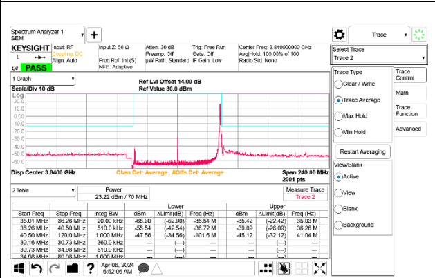
5G NR n77 70MHz BPSK Mid Channel RB1-188 Port B
