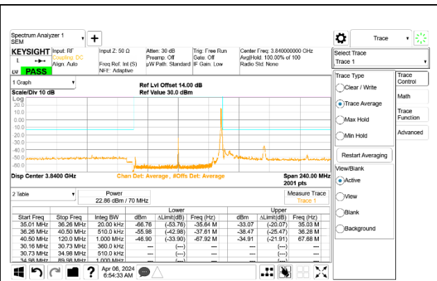
5G NR n77 70MHz BPSK Mid Channel RB1-188 Port A
