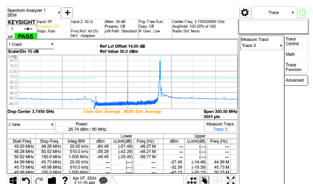
5G NR n77 90MHz BPSK Low Channel RB1-244 Port A+B ID 27342
