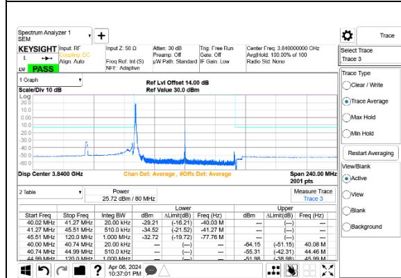
5G NR n77 80MHz BPSK Middle Channel RB1-0 Port A+B
