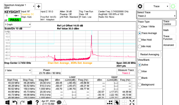
5G NR n77 90MHz BPSK Low Channel RB1-244 Port B ID 27342
