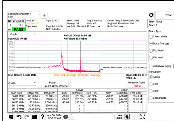
5G NR n77 70MHz BPSK Middle Channel RB1-0 Port B
