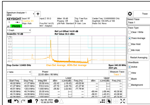
5G NR n77 80MHz BPSK Middle Channel RB1-0 Port A
