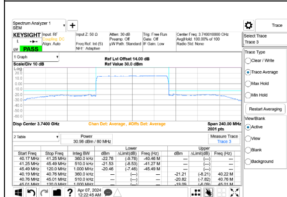
5G NR n77 80MHz BPSK Low Channel RB216-0 Port A+B
