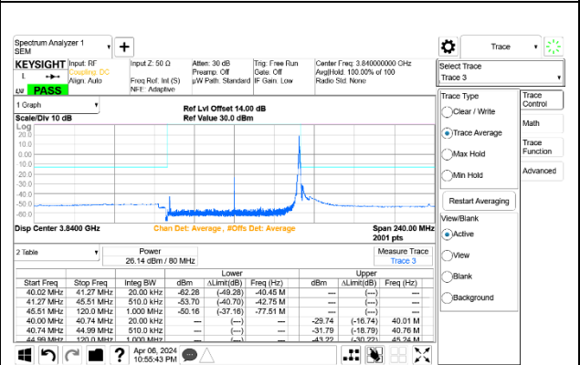
5G NR n77 80MHz BPSK Mid Channel RB1-216 Port A+B
