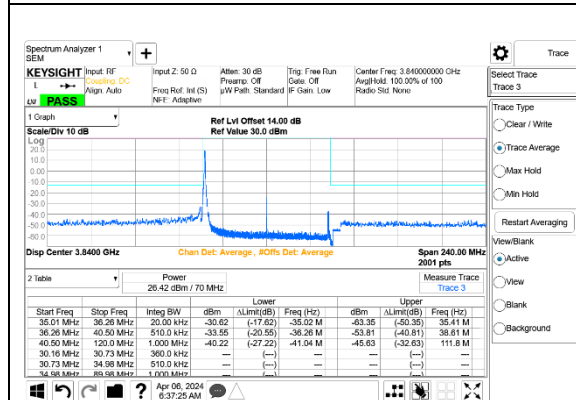
5G NR n77 70MHz BPSK Middle Channel RB1-0 Port A+B
