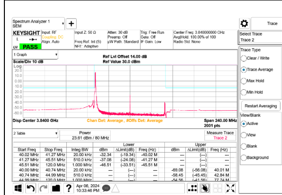
5G NR n77 80MHz BPSK Middle Channel RB1-0 Port B
