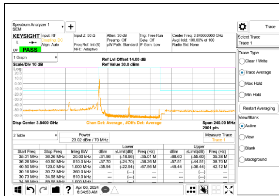
5G NR n77 70MHz BPSK Middle Channel RB1-0 Port A
