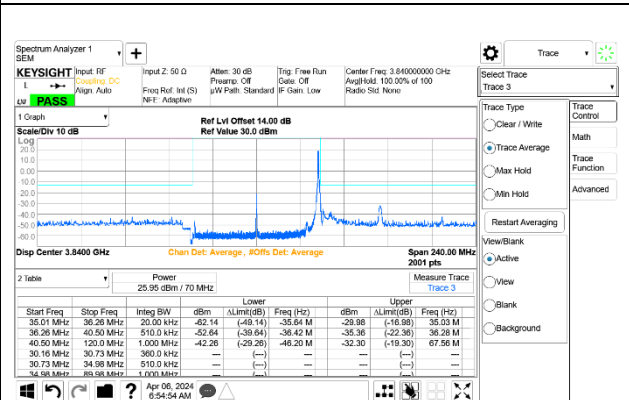
5G NR n77 70MHz BPSK Mid Channel RB1-188 Port A+B
