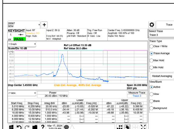
5G NR n77 10MHz BPSK Low Channel RB1-0 Port A+B
