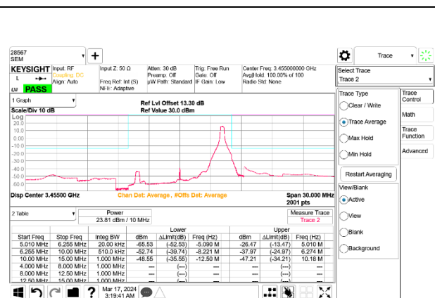
5G NR n77 10MHz BPSK Low Channel RB1-23 Port B
