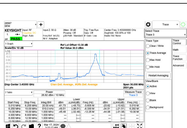
5G NR n77 10MHz BPSK Low Channel RB1-23 Port A+B
