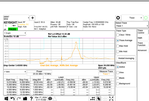
5G NR n77 10MHz BPSK Low Channel RB1-23 Port A
