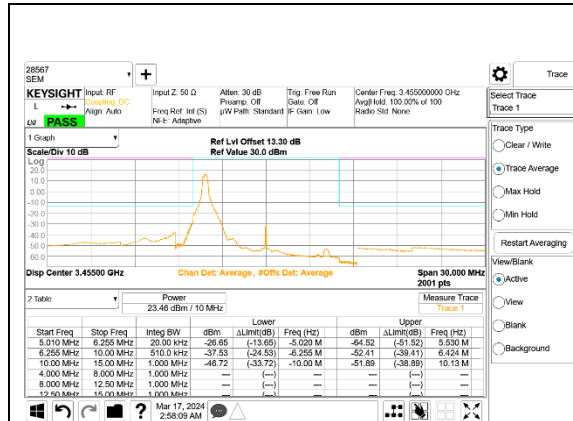
5G NR n77 10MHz BPSK Low Channel RB1-0 Port A
