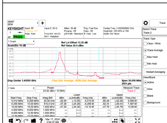
5G NR n77 10MHz BPSK Low Channel RB1-0 Port B
