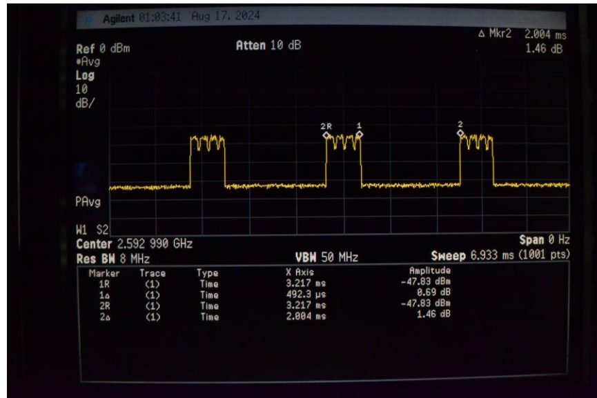
Figure 6: 5G NR TDD Power Class 1.5, 50% RB
