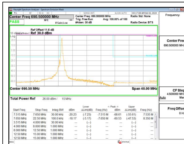
5G NR n71 15MHz BPSK High Channel RB1-0, ID:28567
