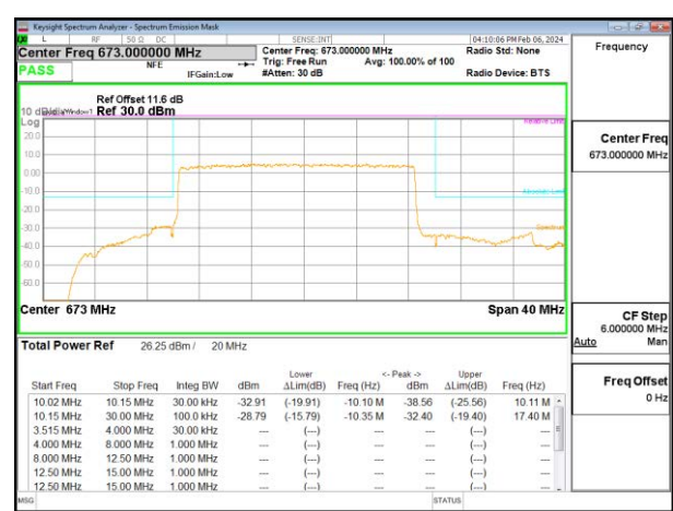
5G NR n71 20MHz BPSK Low Channel RB100-0, ID:28567
