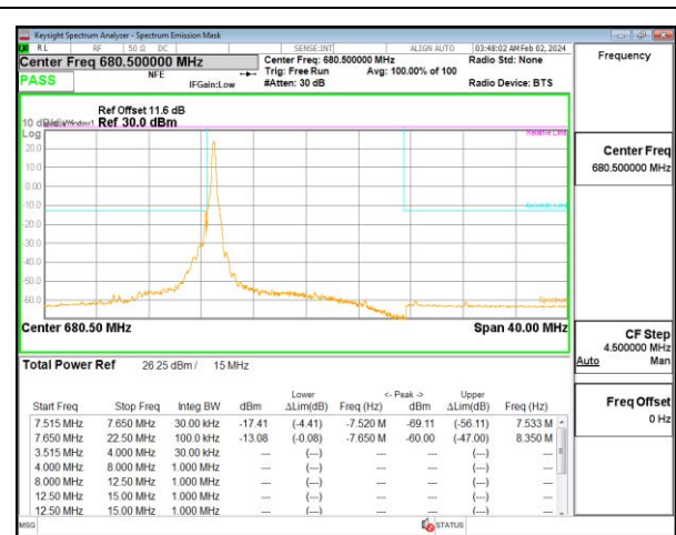
5G NR n71 15MHz BPSK Middle Channel RB1-0, ID:28567
