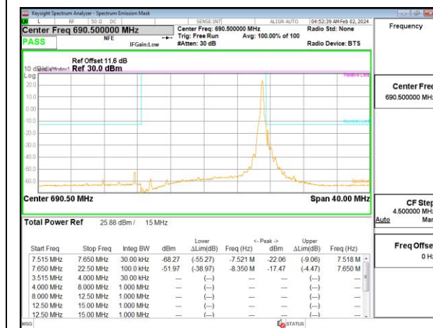
5G NR n71 15MHz BPSK High Channel RB1-78, ID:28567
