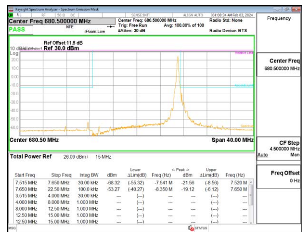
5G NR n71 15MHz BPSK Middle Channel RB1-78, ID:28567
