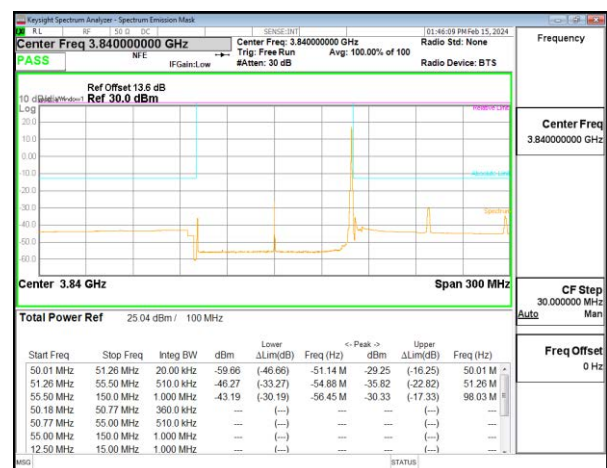
5G NR n77 100MHz BPSK Middle Channel RB1-272, ID:28567
