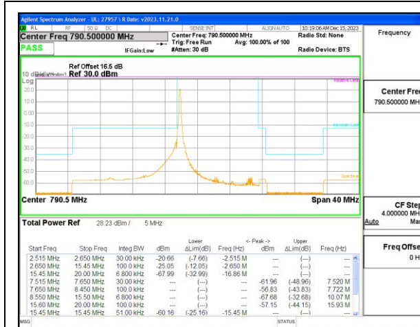
LTE B14 5MHz QPS Low Channel RB1-0
