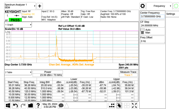
5G NR n77 70MHz BPSK Low Channel RB1-0 Port A ID: 32546
