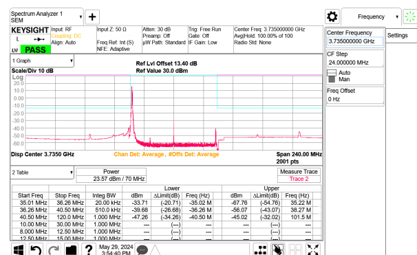
5G NR n77 70MHz BPSK Low Channel RB1-0 Port B ID: 32546
