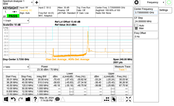
5G NR n77 70MHz BPSK Low Channel RB1-188 Port A ID: 32546
