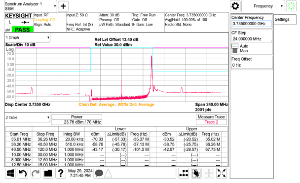
5G NR n77 70MHz BPSK Low Channel RB1-188 Port B ID: 32546
