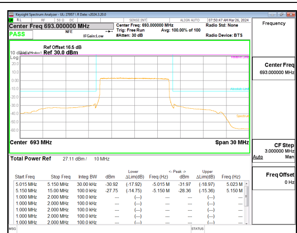
LTE B71 10MHz QPSK High Channel RB50-0
