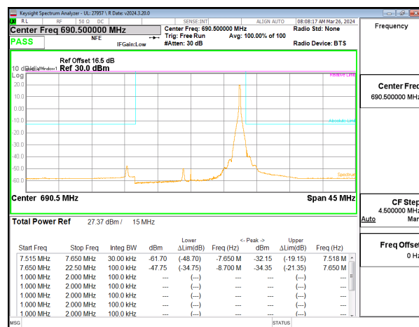
LTE B71 15MHz QPSK High Channel RB1-74
