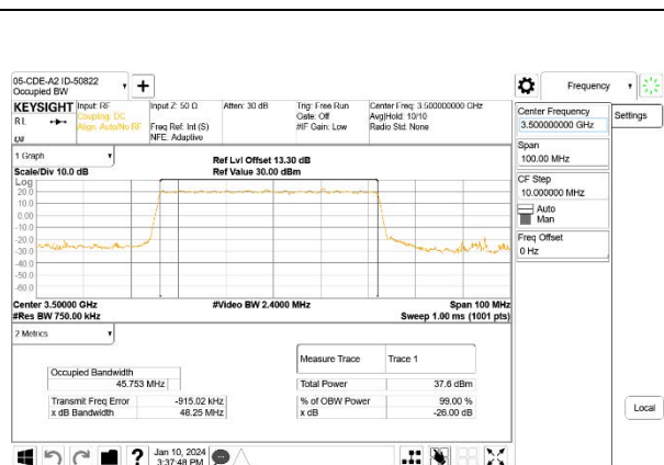
5G NR n77 50MHz BPSK Middle Channel RB128-0
