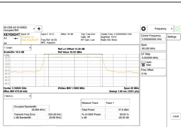
5G NR n77 30MHz BPSK Middle Channel RB75-0
