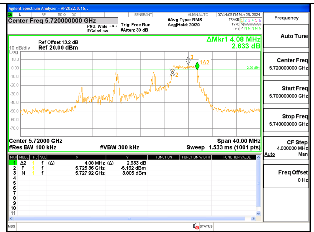
20MHz - Straddle Channel - 52T-RU40 - Ant 6
