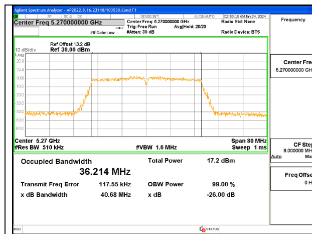
40MHz - Low Channel (UNII-2a) - Ant 6
