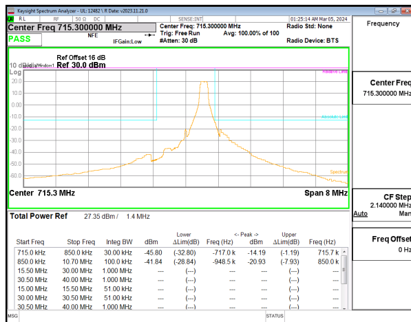
LTE B12 1.4MHz QPSK High Channel RB1-5
