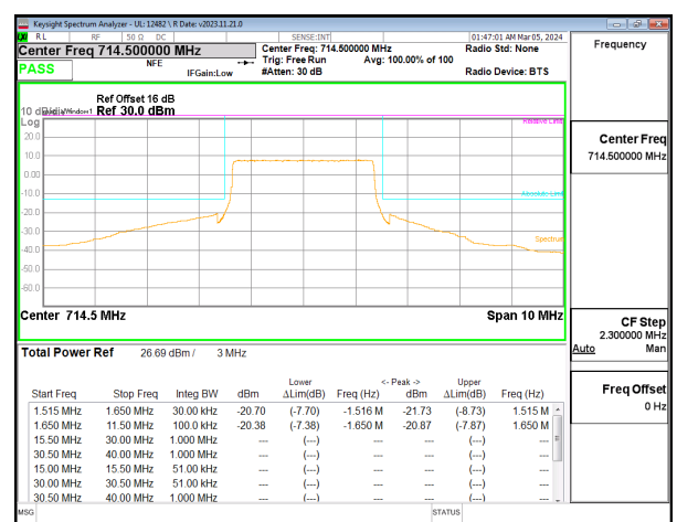
LTE B12 3MHz QPSK High Channel RB15-0
