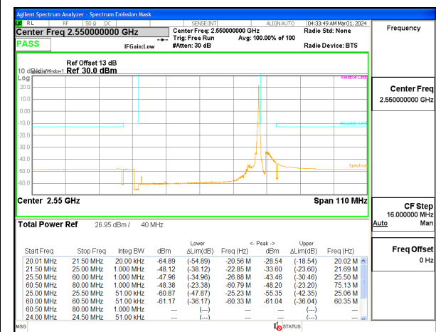
5G NR n7 40MHz BPSK High Channel RB1-215, ID:12482
