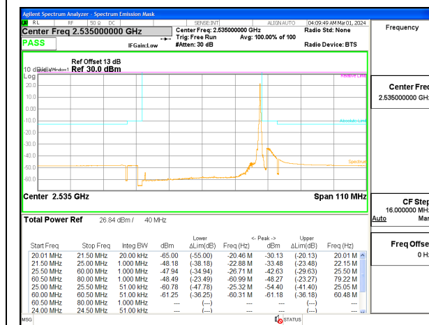
5G NR n7 40MHz BPSK Middle Channel RB1-215, ID:12482
