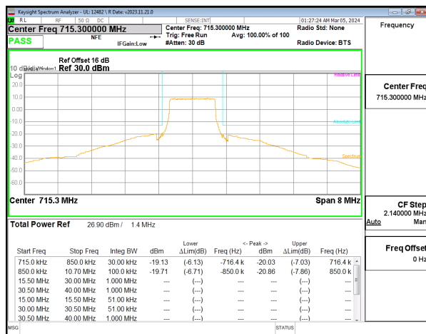
LTE B12 1.4MHz QPSK High Channel RB6-0
