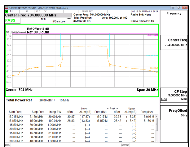
LTE B12 10MHz QPSK Low Channel RB50-0
