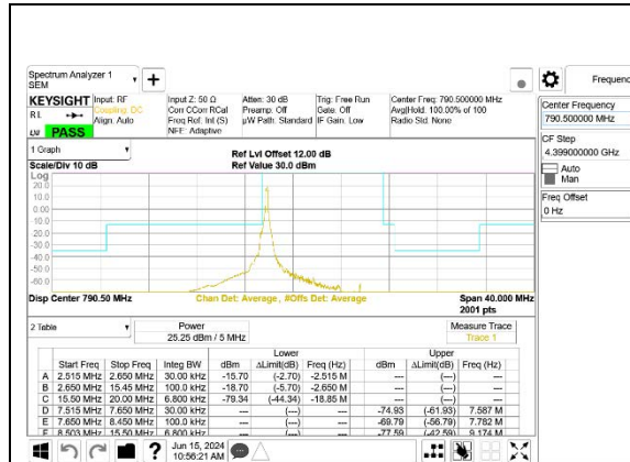
5G NR n14 5MHz BPSK Low Channel RB1-0, ID: 28774
