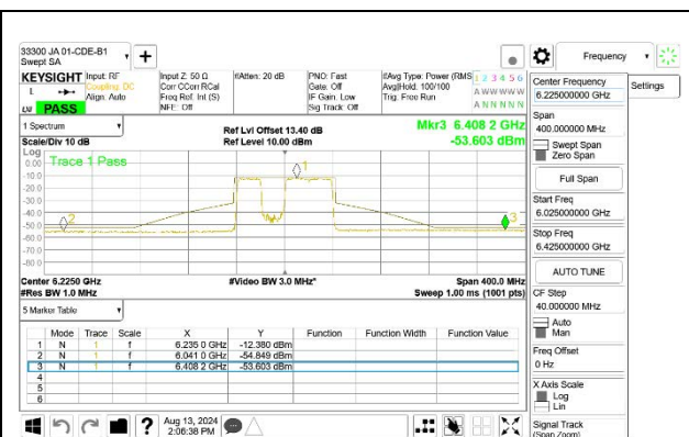
MID CHANNEL, 6225 MHz [ANT 5]
