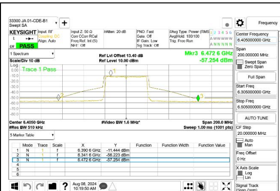
HIGH CHANNEL, 6405 MHz [ANT 5]
