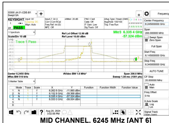
MID CHANNEL, 6245 MHz [ANT 6]
