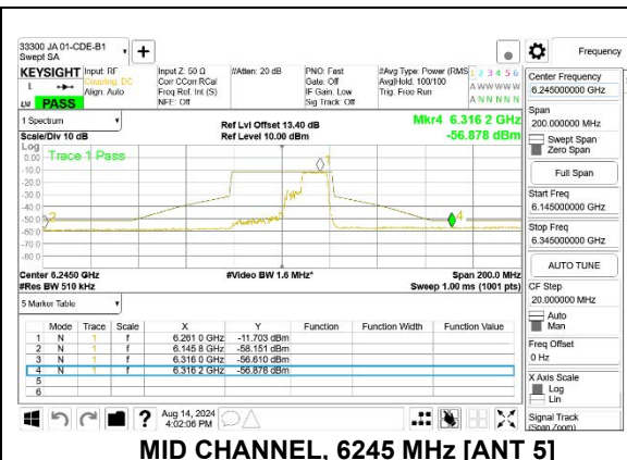
MID CHANNEL, 6245 MHz [ANT 5]
