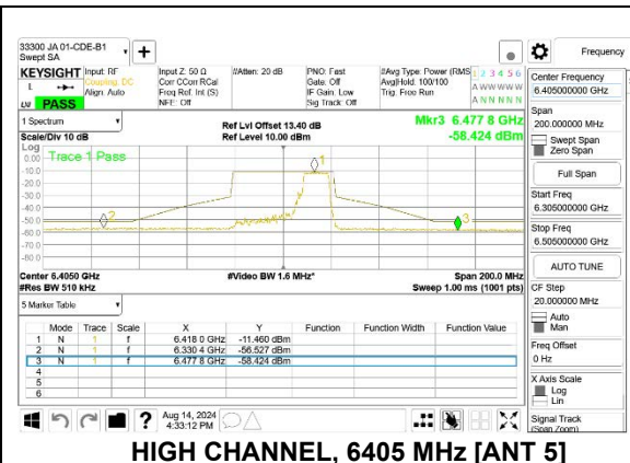
HIGH CHANNEL, 6405 MHz [ANT 5]
