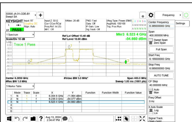
HIGH CHANNEL, 6385 MHz [ANT 5]
