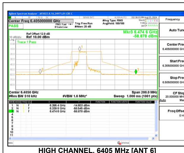
HIGH CHANNEL, 6405 MHz [ANT 6]
