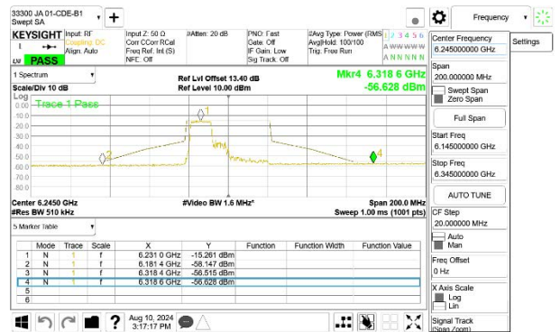
MID CHANNEL, 6245 MHz [ANT 5]
