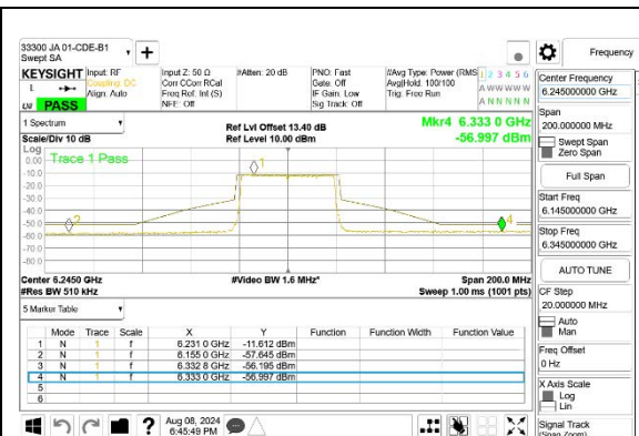
MID CHANNEL, 6245 MHz [ANT 5]
