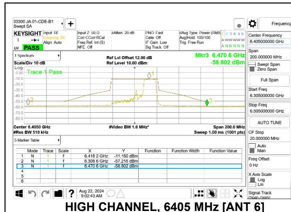
HIGH CHANNEL, 6405 MHz [ANT 6]
