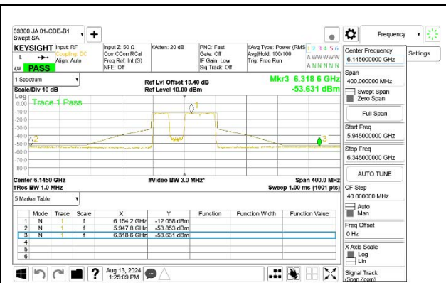
LOW CHANNEL, 6145 MHz [ANT 5]
