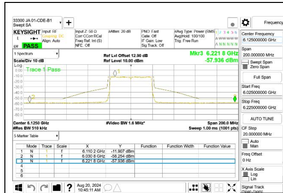
LOW CHANNEL, 6125 MHz [ANT 6]
