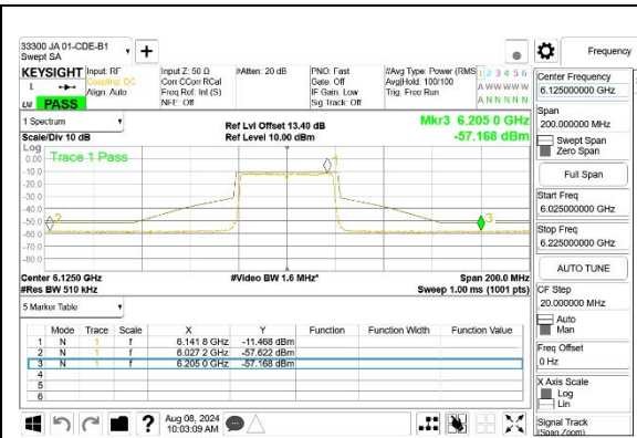
LOW CHANNEL, 6125 MHz [ANT 5]
