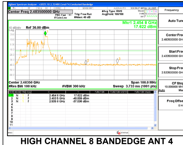
OUT-OF-BAND HIGH CHANNEL 8 ANT 4
