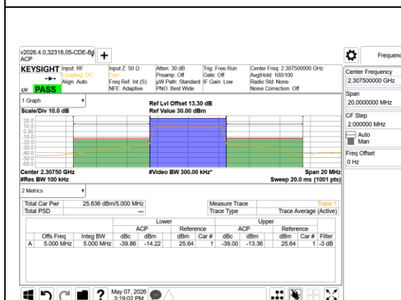
LTE B30 5MHz QPSK Low Channel RB25-0
