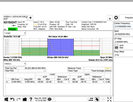
5G NR n30 5MHz BPSK Middle Channel RB1-0
