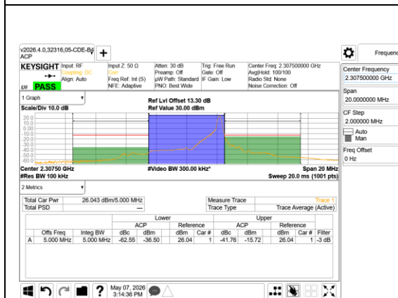
LTE B30 5MHz QPSK Low Channel RB1-24
