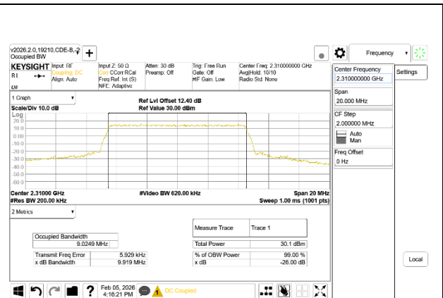
LTE B30 10MHz QPSK Middle Channel RB50-0
