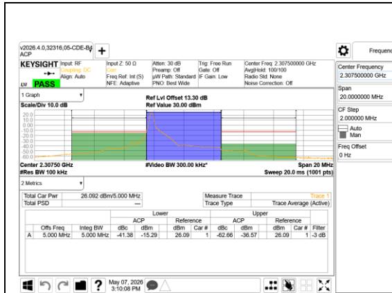
LTE B30 5MHz QPSK Low Channel RB1-0
