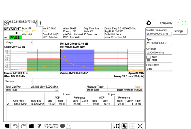
LTE B30 5MHz QPSK Middle Channel RB1-0
