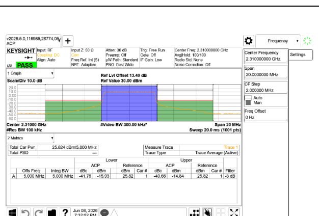
LTE B30 5MHz QPSK Middle Channel RB25-0
