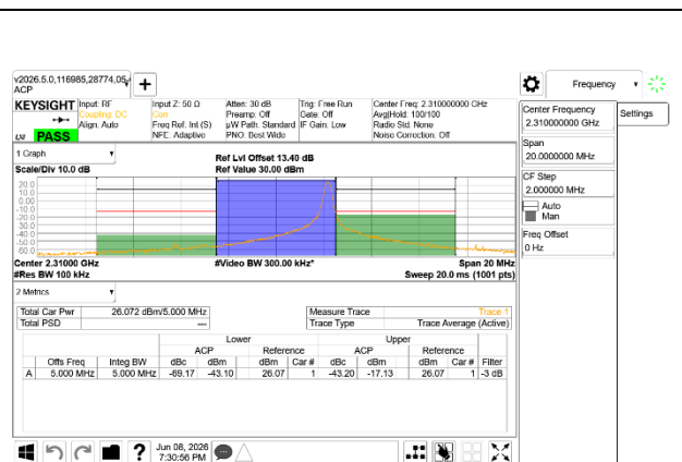
LTE B30 5MHz QPSK Middle Channel RB1-24
