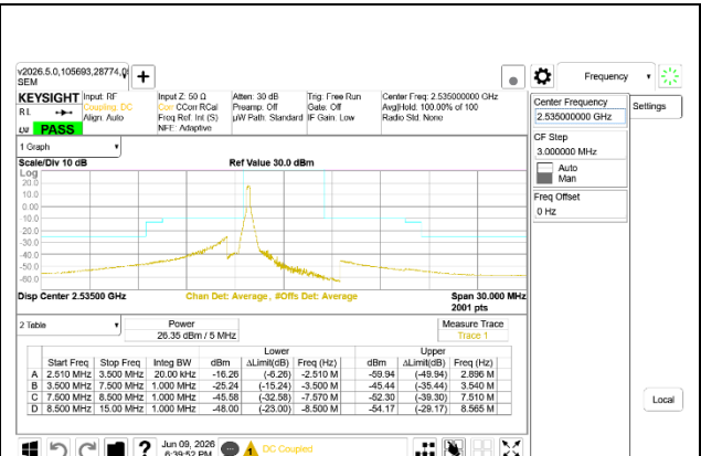
5G NR n7 5MHz BPSK Middle Channel RB1-0
