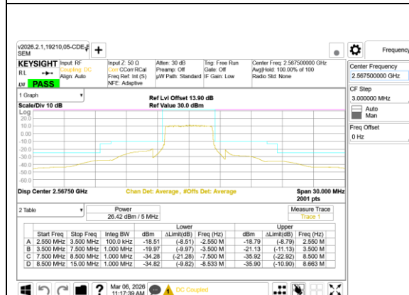
LTE B7 5MHz QPSK High Channel RB25-0
