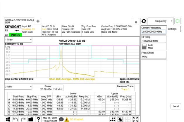
LTE B7 10MHz QPSK Low Channel RB1-0
