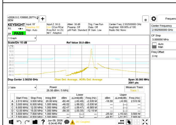
5G NR n7 5MHz BPSK Low Channel RB1-24
