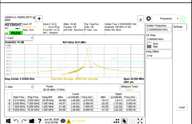
5G NR n7 5MHz BPSK Middle Channel RB1-24
