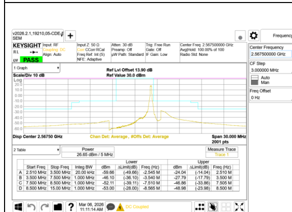
LTE B7 5MHz QPSK High Channel RB1-24
