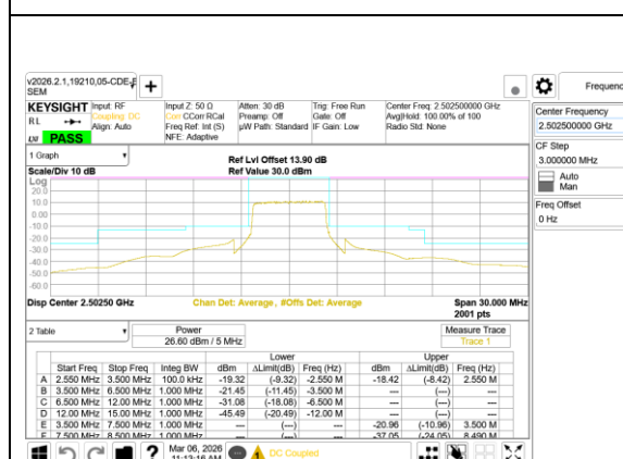
LTE B7 5MHz QPSK Low Channel RB25-0
