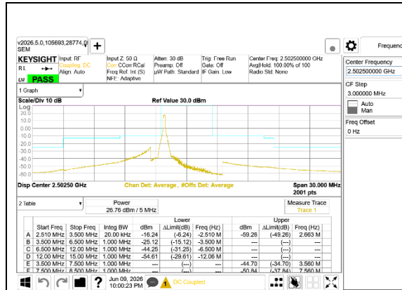
5G NR n7 5MHz BPSK Low Channel RB1-0
