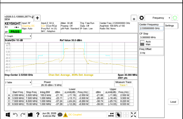
5G NR n7 5MHz BPSK Middle Channel RB25-0
