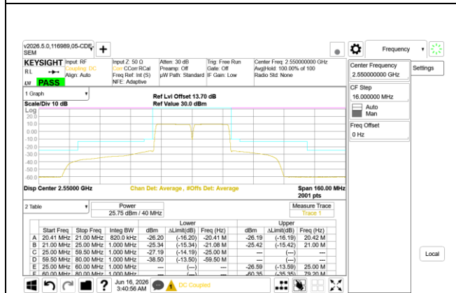
ULCA LTE B7 20MHz + 20MHz QPSK High Ch RB100-0 + RB100-0
