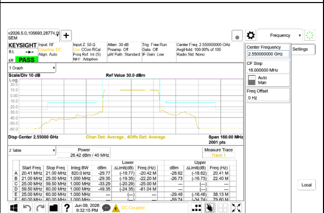
5G NR n7 40MHz BPSK High Channel RB216-0
