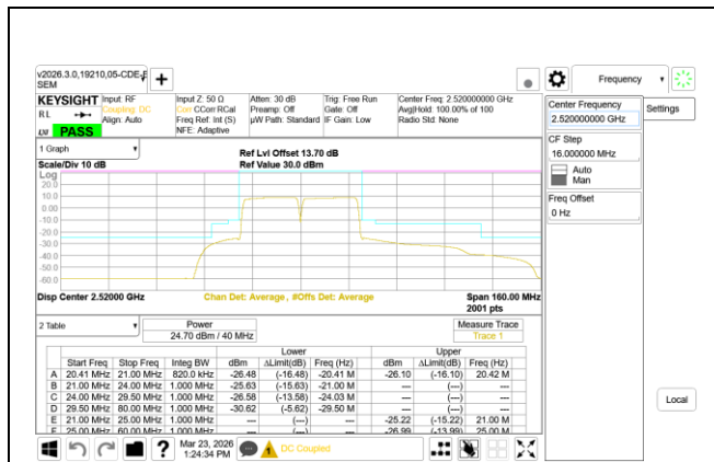
ULCA LTE B7 20MHz + 20MHz QPSK Low Ch RB100-0 + RB100-0
