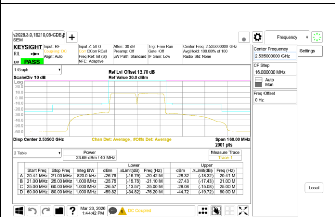
ULCA LTE B7 20MHz + 20MHz 16QAM Mid Ch RB100-0 + RB100-0
