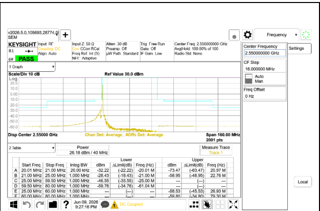
5G NR n7 40MHz BPSK High Channel RB1-0
