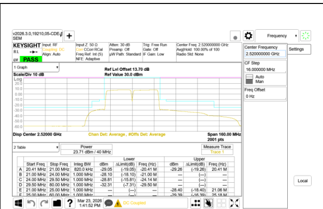
ULCA LTE B7 20MHz + 20MHz 16QAM Low Ch RB100-0 + RB100-0
