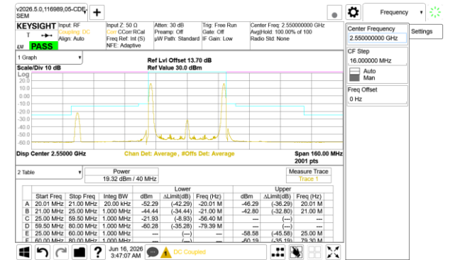
ULCA LTE B7 20MHz + 20MHz 16QAM High Ch RB1-0 + RB1-99
