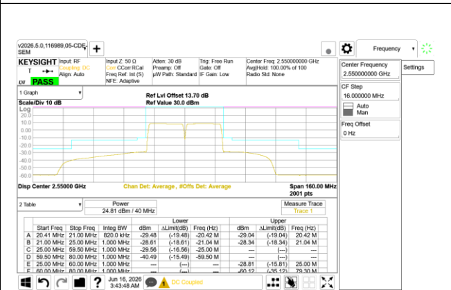
ULCA LTE B7 20MHz + 20MHz 16QAM High Ch RB100-0 + RB100-0
