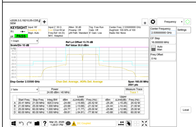
ULCA LTE B7 20MHz + 20MHz QPSK Mid Ch RB100-0 + RB100-0
