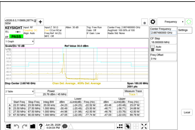
5G NR n41 45MHz BPSK High Channel RB1-0
