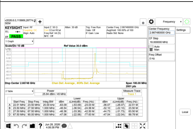
5G NR n41 45MHz BPSK High Channel RB1-118
