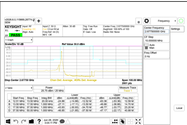
5G NR n41 25MHz BPSK High Channel RB1-0
