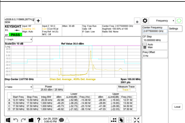
5G NR n41 25MHz BPSK High Channel RB1-64
