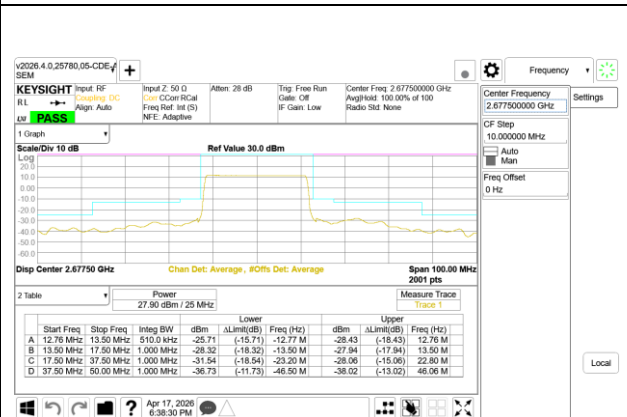
5G NR n41 25MHz BPSK High Channel RB64-0
