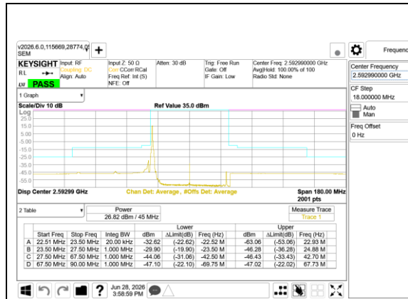
5G NR n41 45MHz BPSK Middle Channel RB1-0
