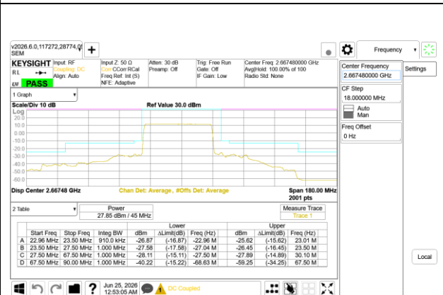
5G NR n41 45MHz BPSK High Channel RB108-0
