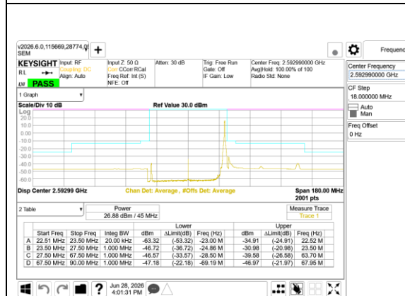
5G NR n41 45MHz BPSK Middle Channel RB1-118
